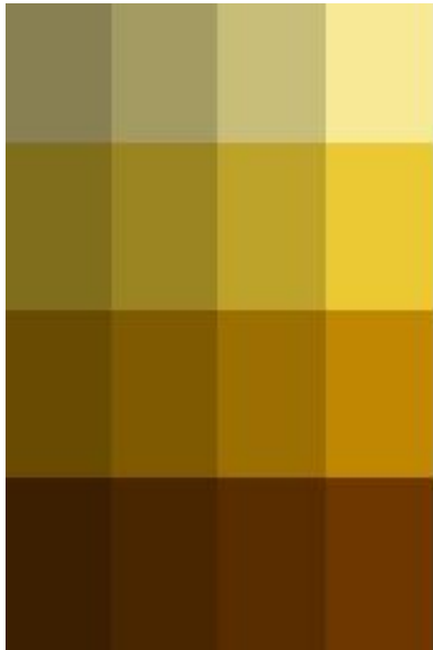
potassium perchlorate
