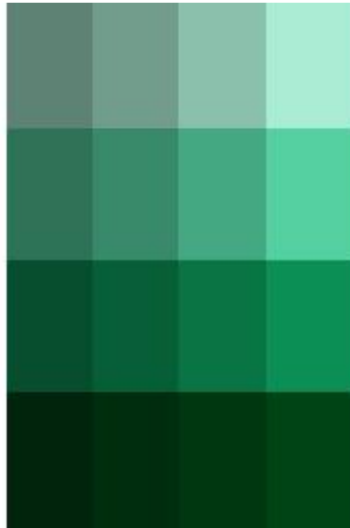
nickel manganate
