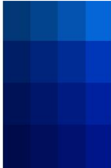
cobalt chloride
