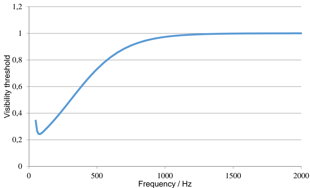
Figure 4 – SVM sensitivity curve
